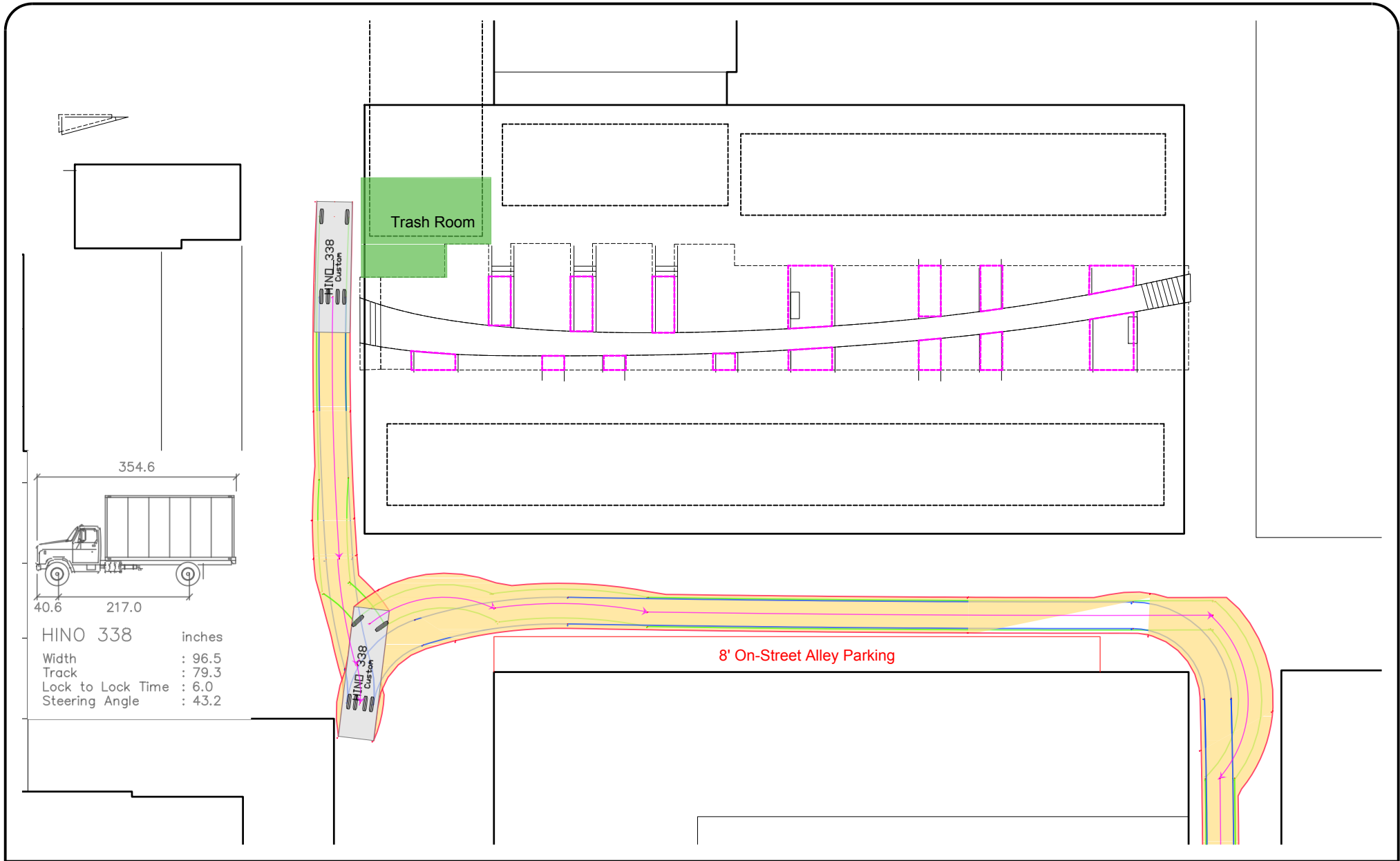
Figure 2 Truck Sweep Diagram - Rear Load Trash Truck Egress
