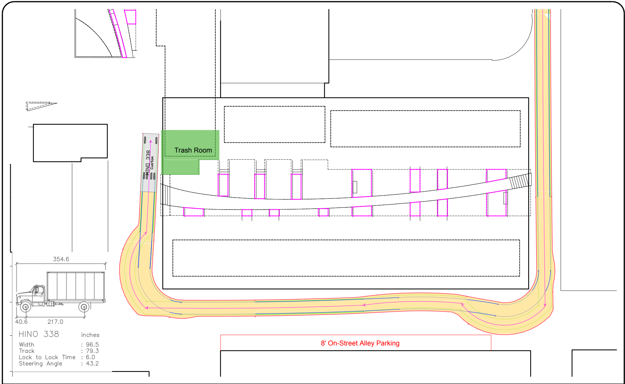
Figure 1 Truck Sweep Diagram - Rear Load Trash Truck Ingress
